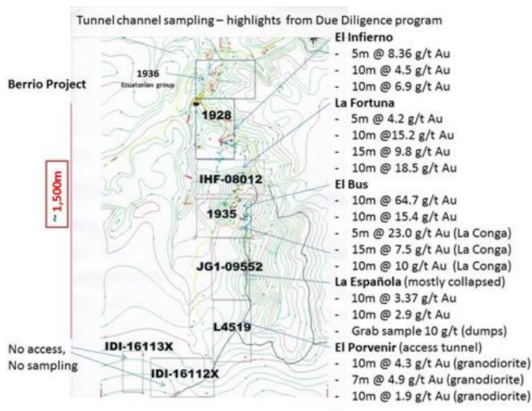
Figure 2: Highlights of tunnel channel sampling program
