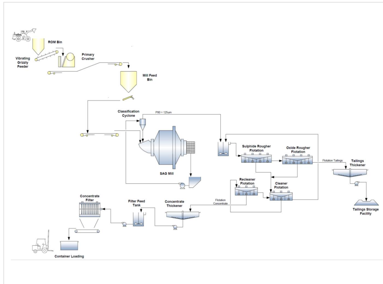
Image: Sorby Hills processing circuit
