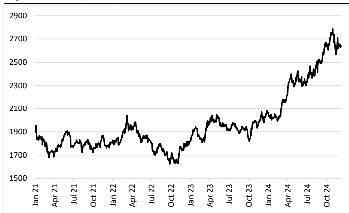
Figure 3: Gold (US$/oz)
