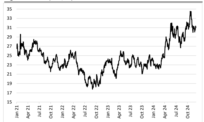
Figure 4: Silver (US$/oz)
