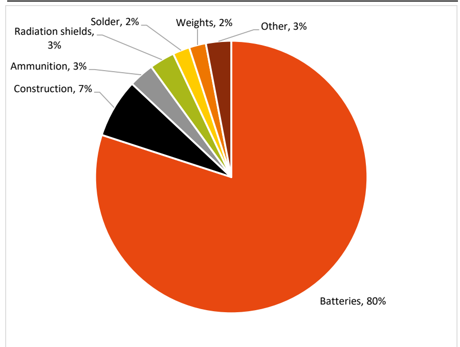
Figure 9: Lead usage 2023
